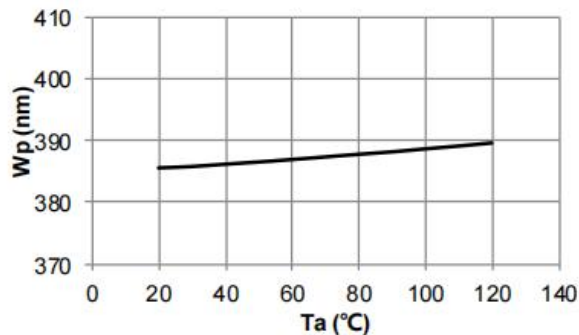
Fig.5- Peak Wavelength (@500mA) vs. Ambient Temperature
