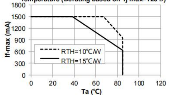
Fig.6-Maximum Driving Forward DC Current vs. Ambient Temperature (Derating based on T_J \text{ max}=125^\circ\text{C} )
