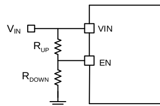
Figure 11: Adjustable UVLO Using EN Divider
