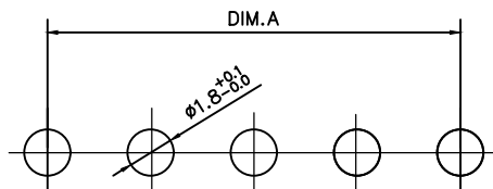
PCB LAYOUT
