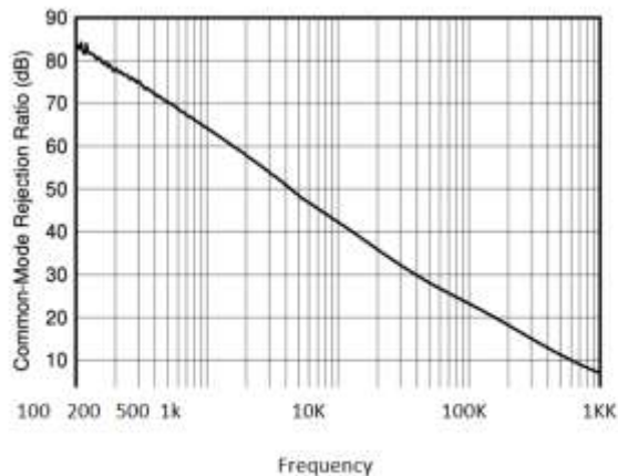
Figure 3. CMRR vs Frequency
