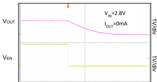
Shutdown from EN ( V_{OUT}=1.8V )
