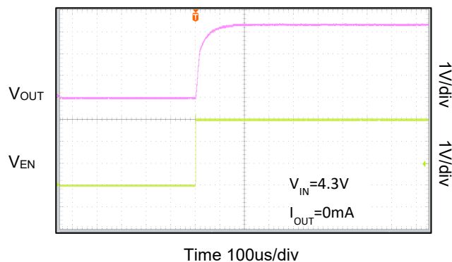
Start up from EN ( V_{OUT}=3.3V )
