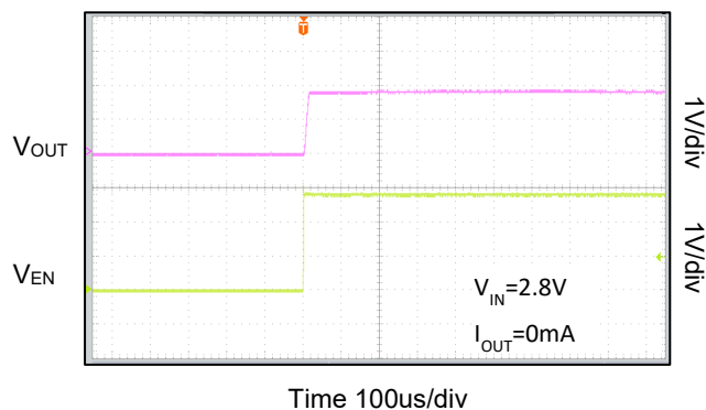
Start up from EN ( V_{OUT}=1.8V )
