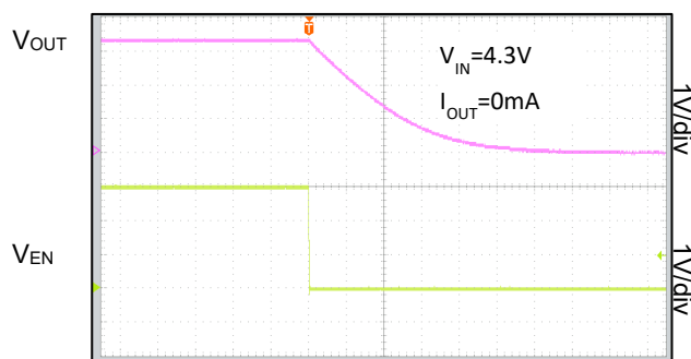
Shutdown from EN ( V_{OUT}=3.3V )
