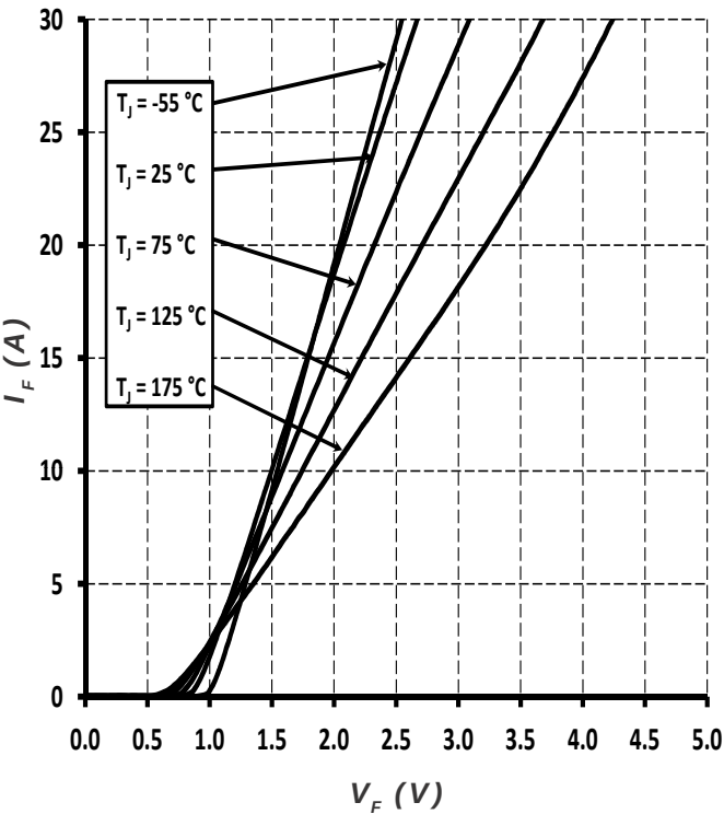
Figure 1. Forward Characteristics
