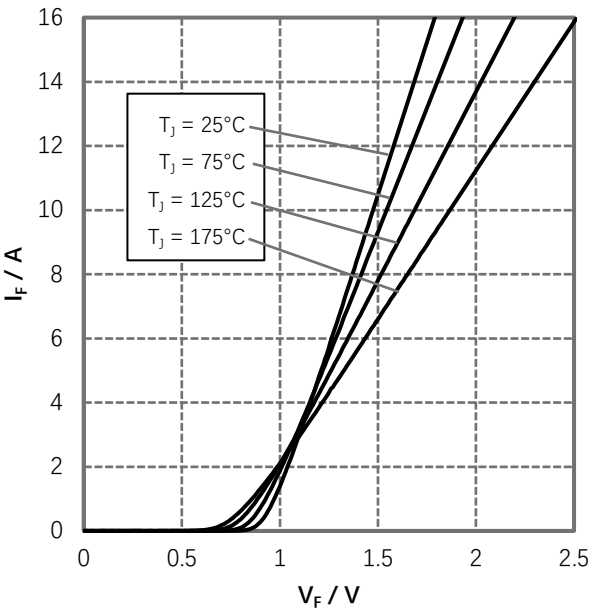
Figure 1. Forward Characteristics
