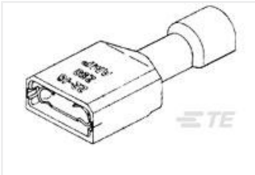
TE Part #3-520117-2 ULTRAFAST 250 ASSY REC 16-14 TPBR LP
