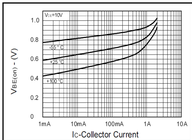
Figure 5 : V_{BE(on)}-I_C
