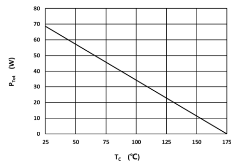
Fig 4: Power Derating
