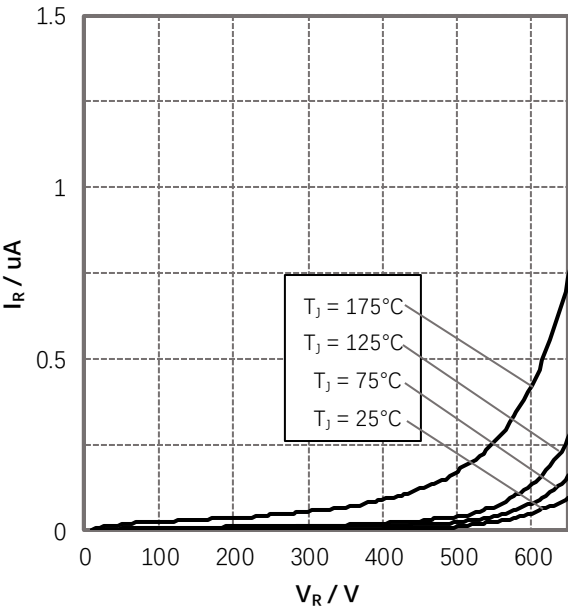
Figure 2. Reverse Characteristics
