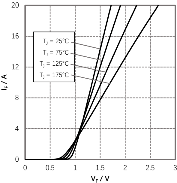
Figure 1. Forward Characteristics
