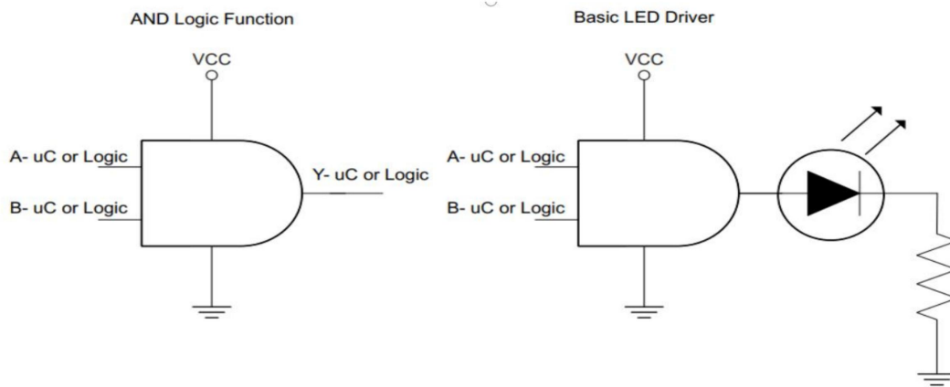
Figure 5.1: Application Schematic
