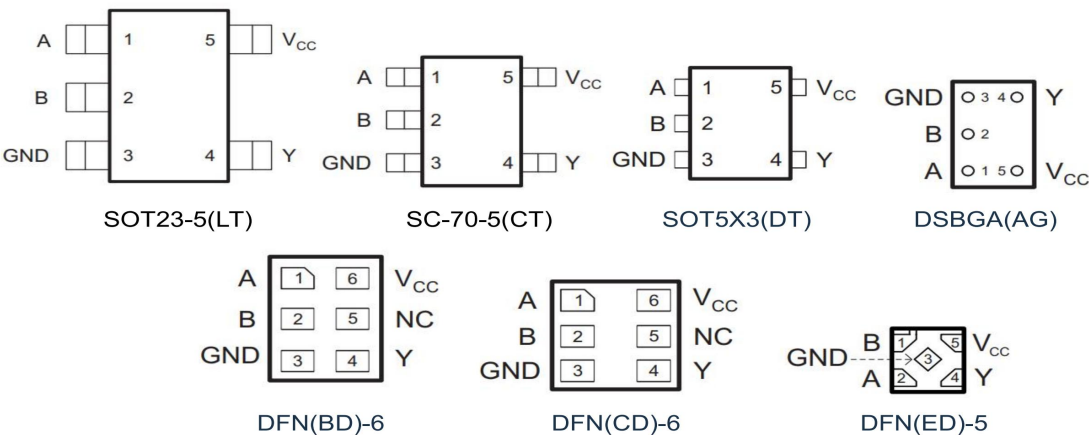
Figure 2.1: Top View
