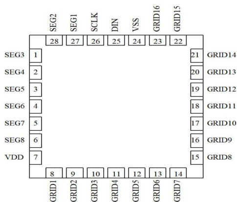
HTM1640 QFN28(4*4)
