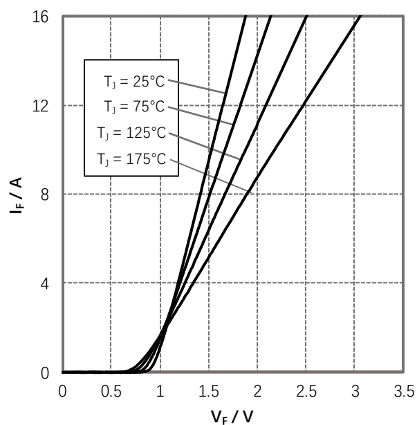
Figure 1. Forward Characteristics
