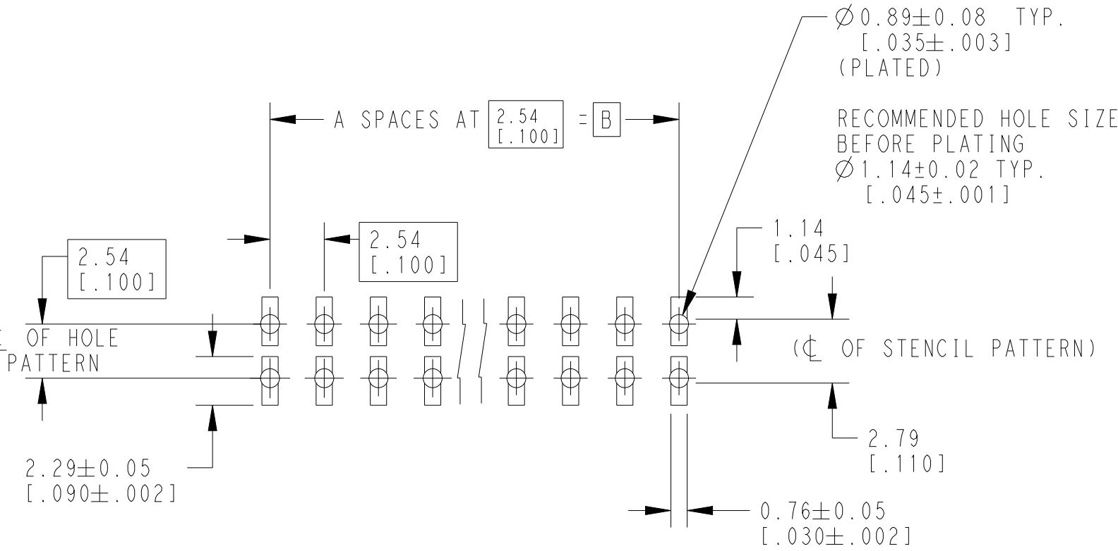
RECOMMENDED PC BOARD MOUNTING DIMENSIONS FOR 1.60[.063] THICK PC BOARD AND .305[.012] STENCIL THICK
