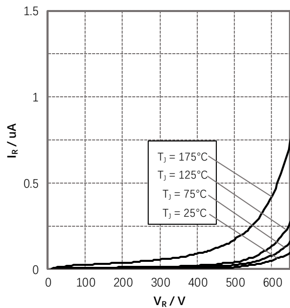
Figure 2. Reverse Characteristics
