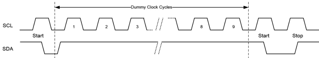
Figure 4-4 Soft Reset
