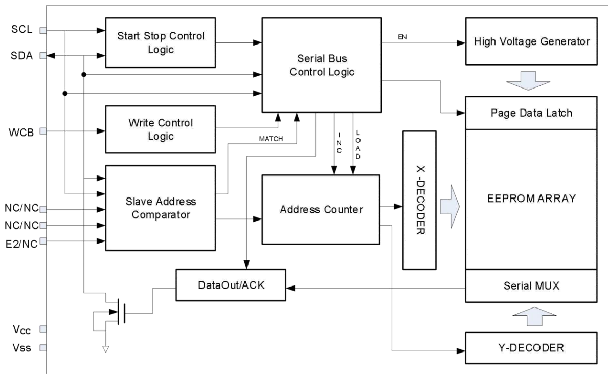
Figure 2-1 Block Diagram
