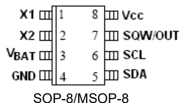
SOP-8/MSOP-8
