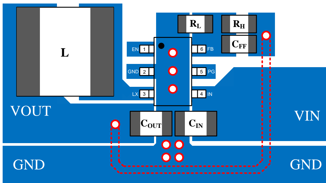
Figure4. PCB Layout Suggestion
