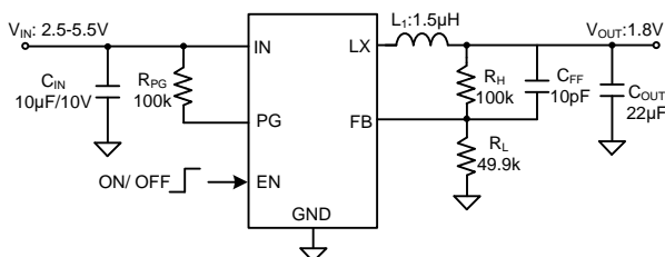
Figure1. Schematic Diagram
