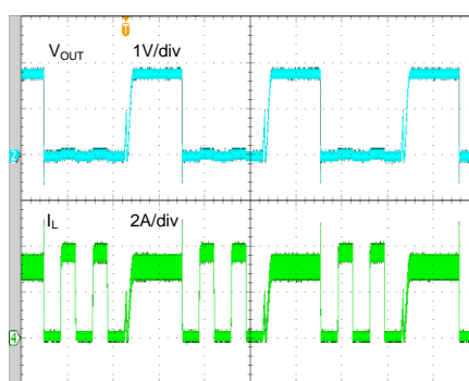
Short Circuit Protection ( V_{IN}=5.0V , V_{OUT}=1.8V , I_O=3A \sim Short)
