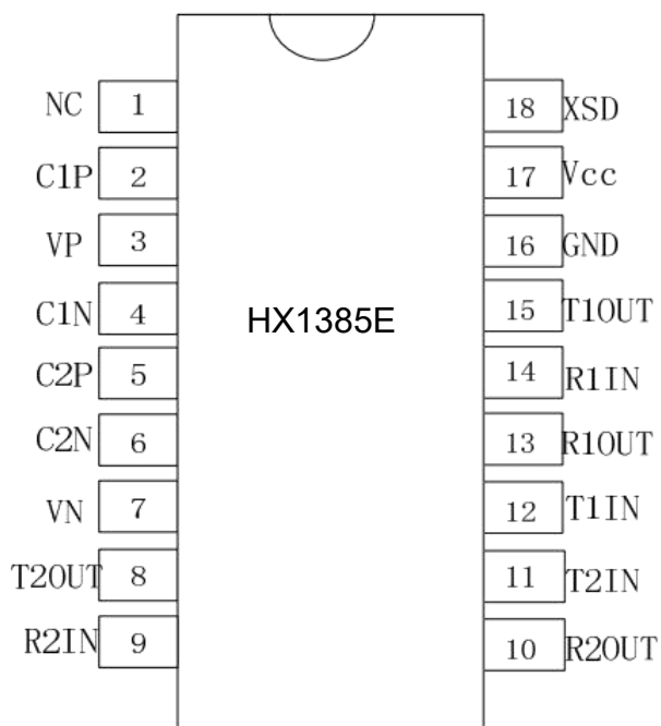
18-pin SOP
