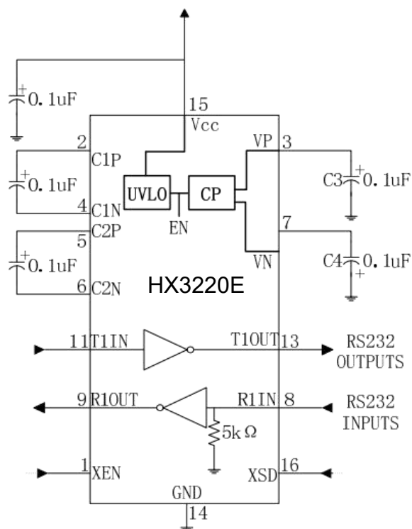
16-pin SOP/TSSOP/SSOP
