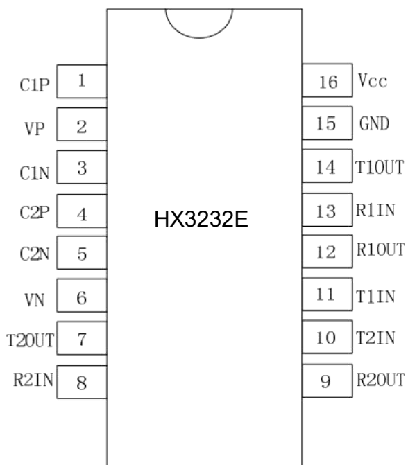
16-pin SOP/TSSOP/SSOP/DIP
