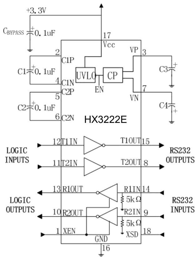
18-pin SOP/DIP
