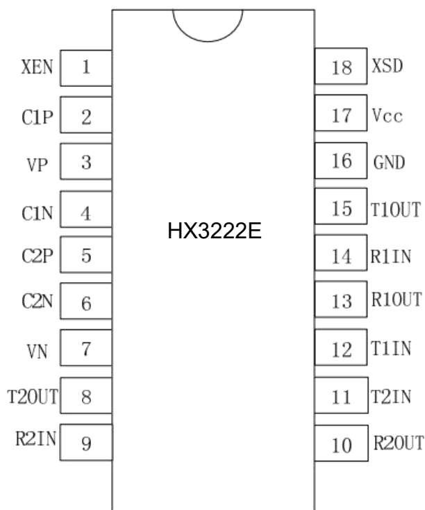
18-pin SOP/DIP
