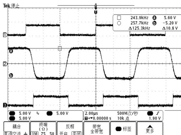
Figure 2.HX32xxE TxIN to TxOUT(loopback to Rx with 1000pF load) at 250Kbps waveform Waveform
