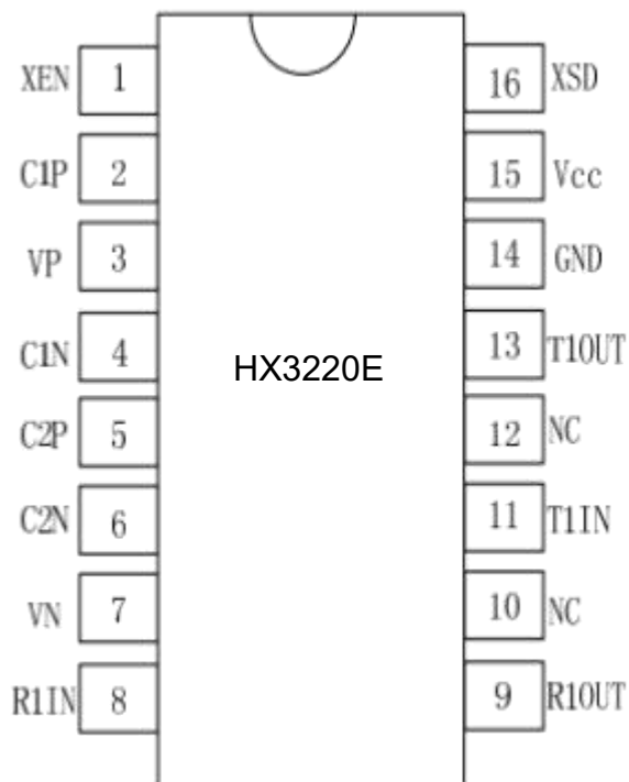
16-pin SOP/TSSOP/SSOP
