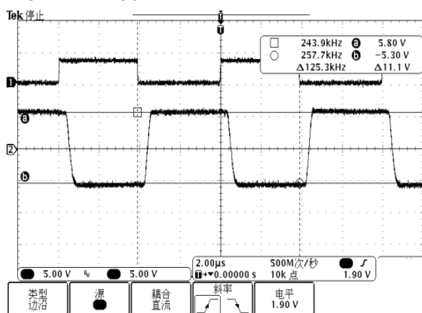
Figure 1.HX32xxE TxIN to TxOUT(no load) at 250kbps
