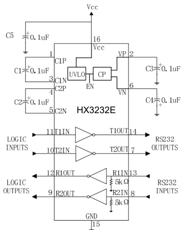
16-pin SOP/TSSOP/SSOP/DIP
