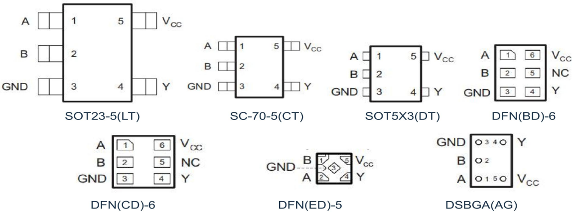
Figure 2.1 Top View
