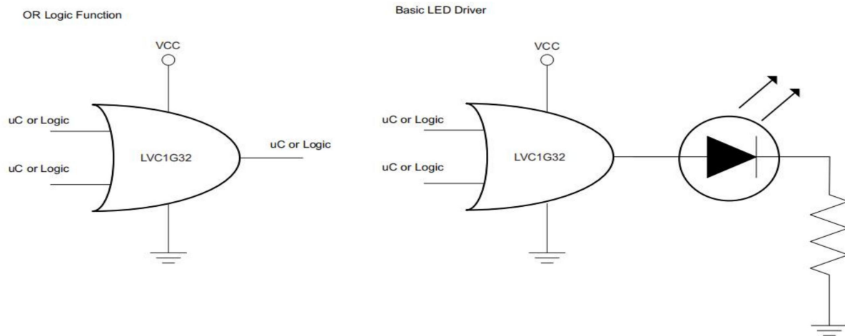
Figure 5.1: Application Schematic
