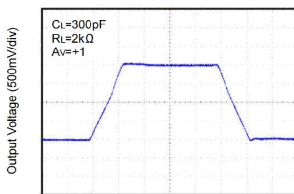
Large Signal Transient Response at +2.5V
