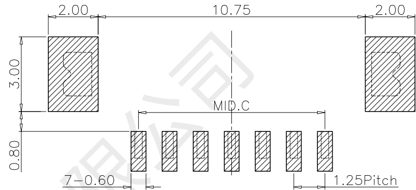
RECOMMENDER P.C.B LAYOUT TOP VIEW (GENERAY TOLERANCE \pm 0.10 )
