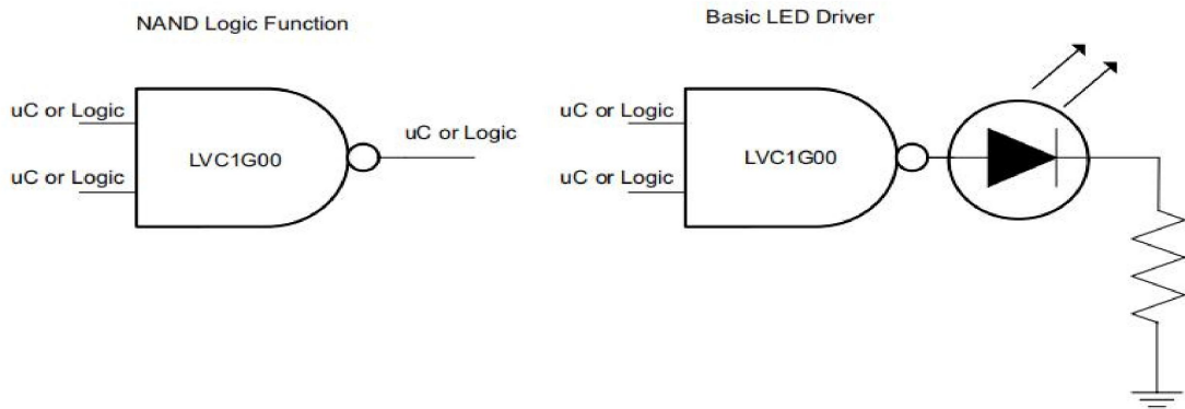
Figure 5.1: Application Schematic
