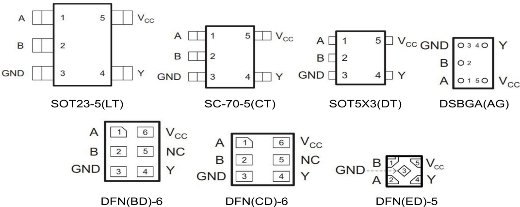
Figure 2.1: Top View
