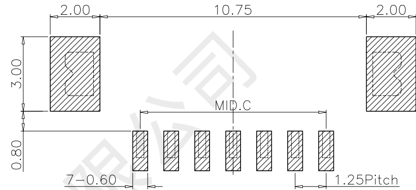
RECOMMENDER P.C.B LAYOUT TOP VIEW (GENERAY TOLERANCE ±0.10)
