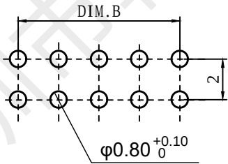
PCB LAYOUT
