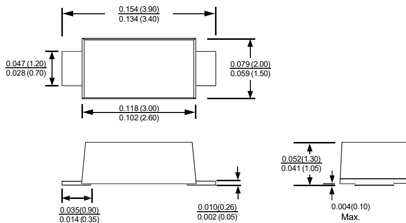
SOD-123FL
