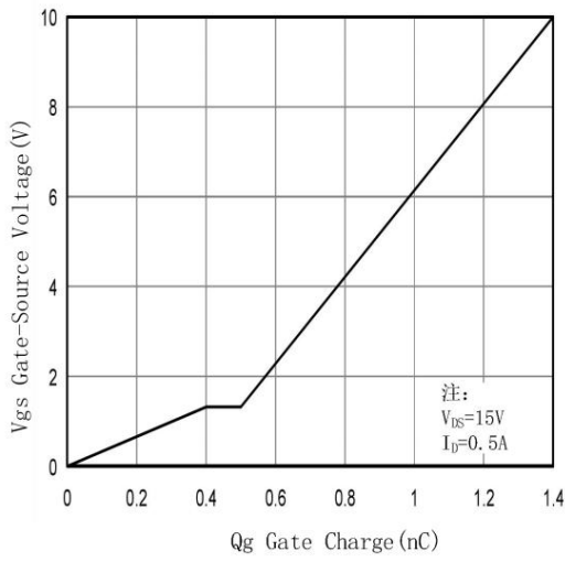
Fig.7 Gate-Charge Characteristic
