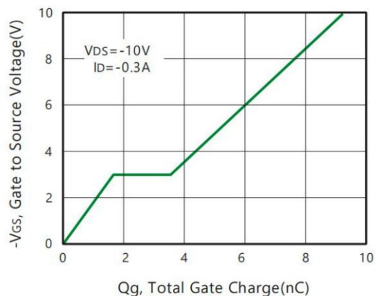
Figure 6. Gate Charge
