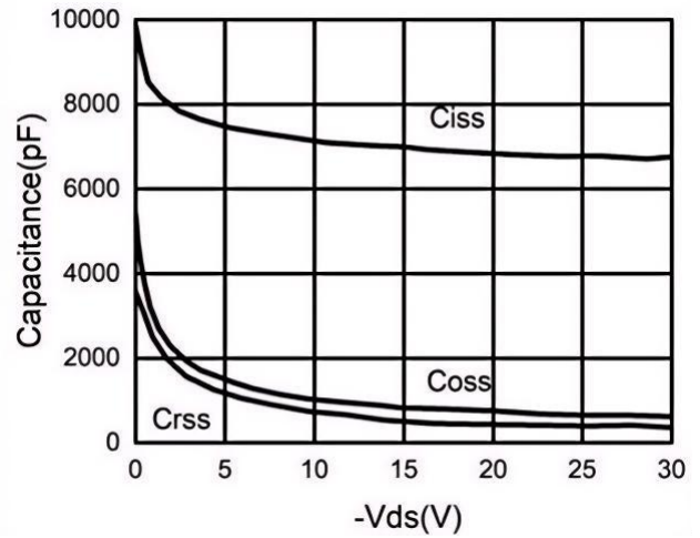
Fig.8 Capacitance
