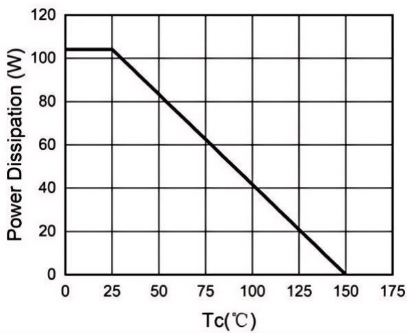
Fig.3 Power Dissipation
