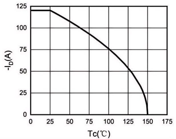
Fig.4 Drain Current
