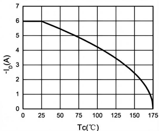
Fig.4 Drain Current
