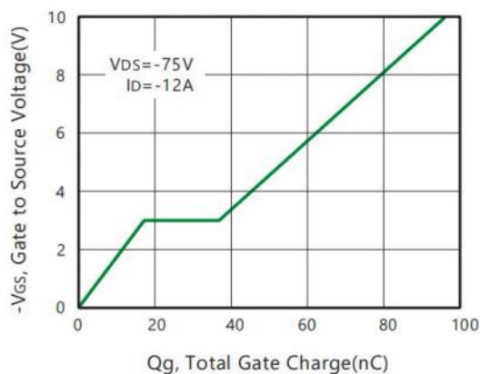
Figure 6. Gate Charge
