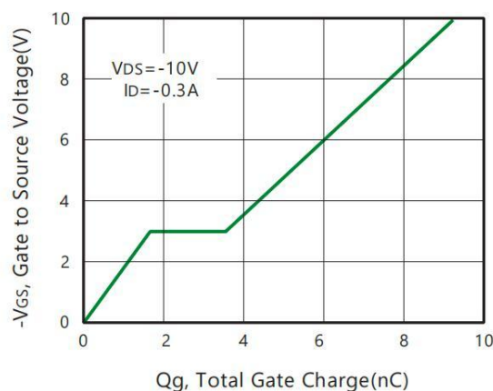
Figure 6. Gate Charge
