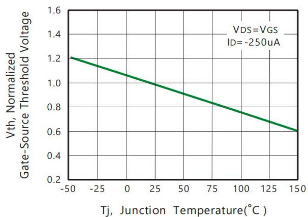
Figure 5. Gate Threshold Variation with Temperature
