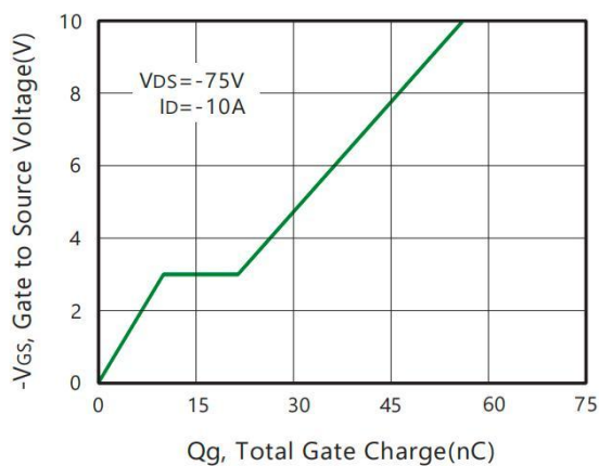
Figure 6. Gate Charge
