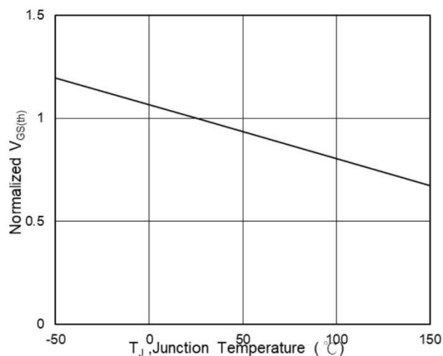
Fig.5 Normalized V_{TH} vs T_J
