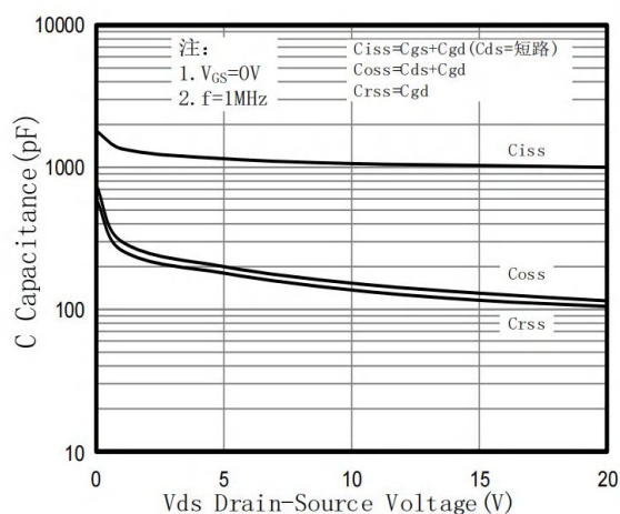
Fig.6 Capacitance Characteristic
