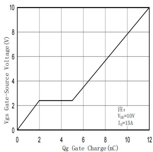
Fig.7 Gate-Charge Characteristic
