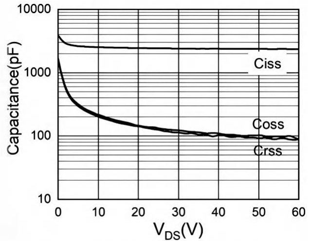
Figure 8. Capacitance
