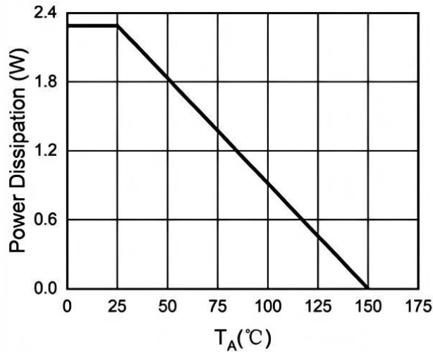
Figure 3. Power Dissipation
