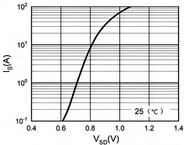
Figure 9. Body-Diode Characteristics
