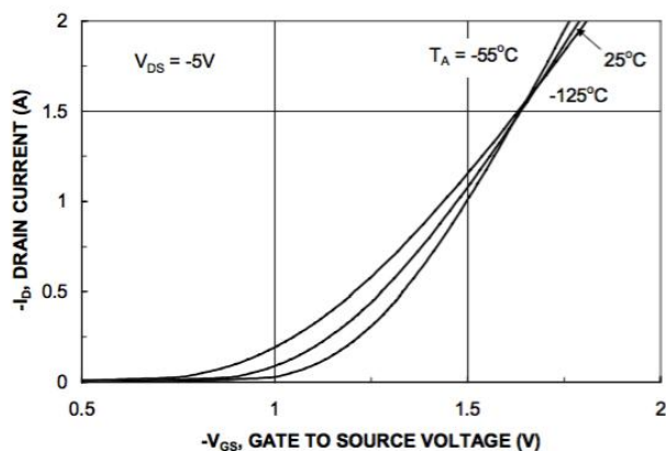
Figure 5. Transfer Characteristics.
