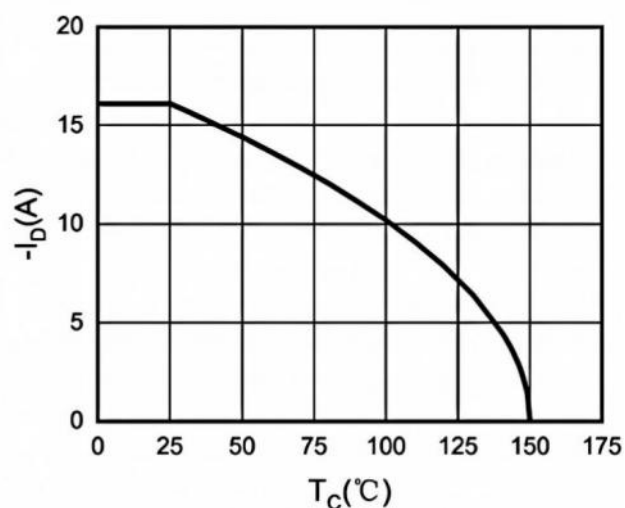
Fig.4 Drain Current
