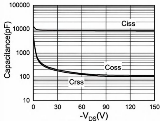
Fig.8 Capacitance
