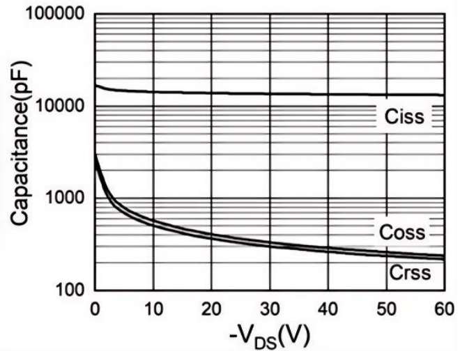
Fig.8 Capacitance
