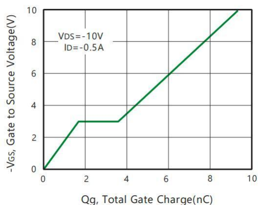
Figure 6. Gate Charge
