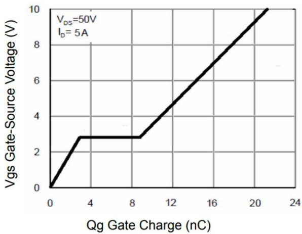
Fig.7 Gate-Charge Characteristic
