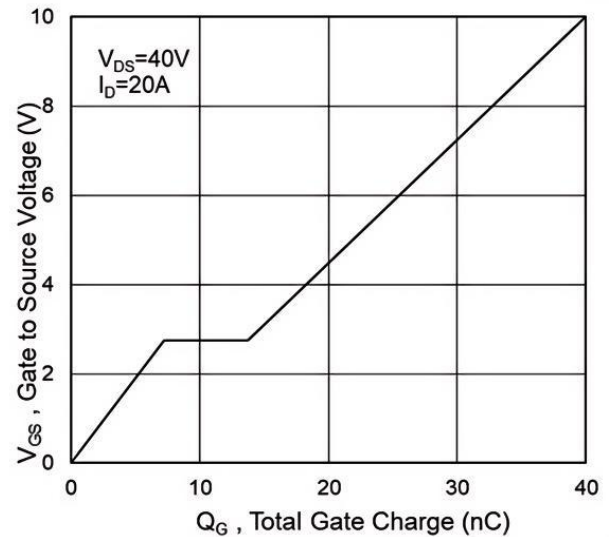
Fig.4 Gate-Charge Characteristics
