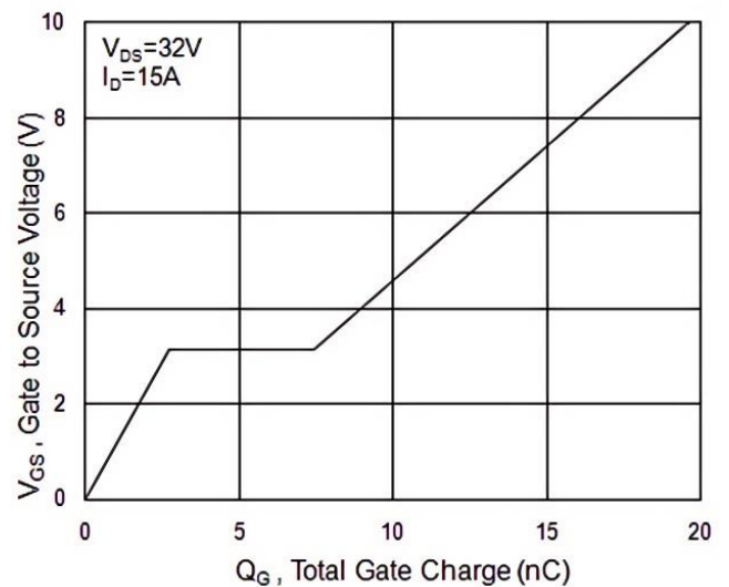
Fig.4 Gate-Charge Characteristics
