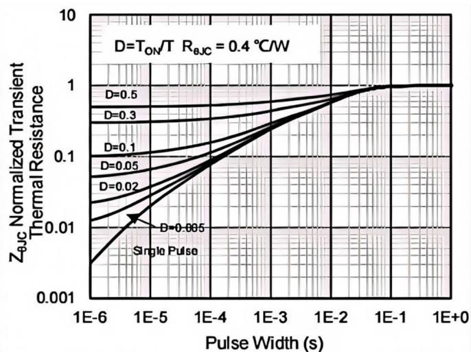
Fig.12 Transient Thermal Response Curve
