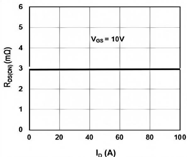
Fig.3 On-Resistance Variation vs Drain Current
