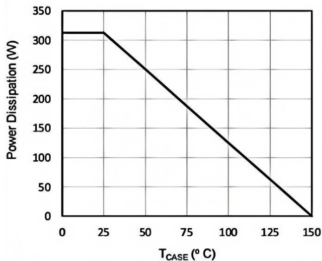
Fig.5 Power Dissipation
