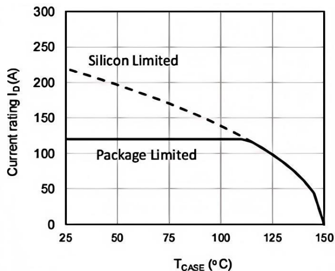
Fig.6 Drain Current Derating
