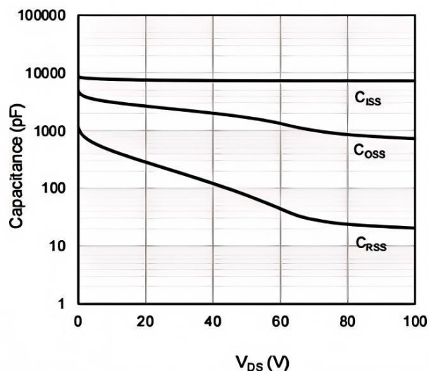
Fig.8 Capacitance
