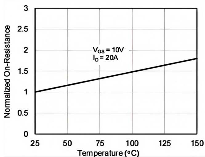
Fig.11 On-Resistance Variation vs Temperature
