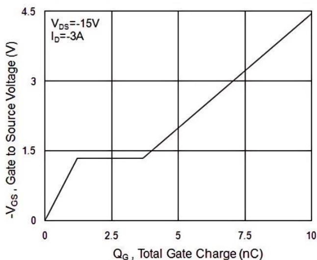
Fig.4 Gate-Charge Characteristics
