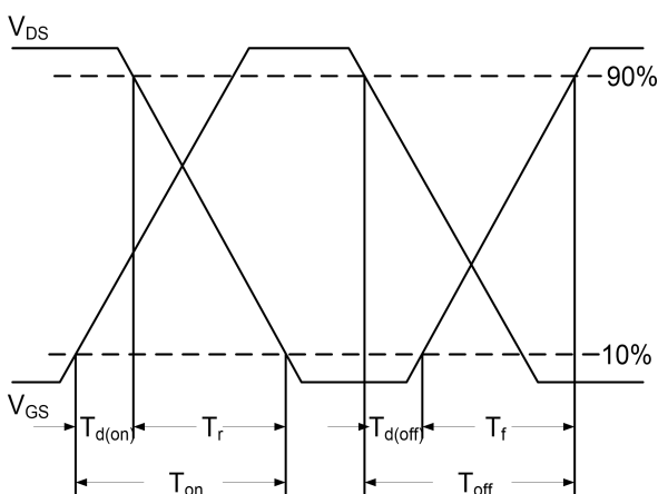
Fig.10 Switching Time ZWaveform
