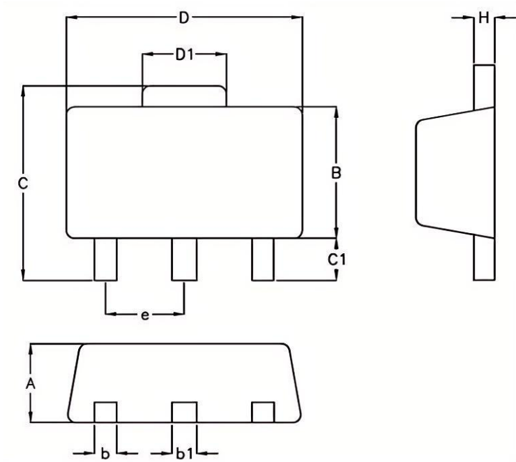
SOT-89 Package Outline
