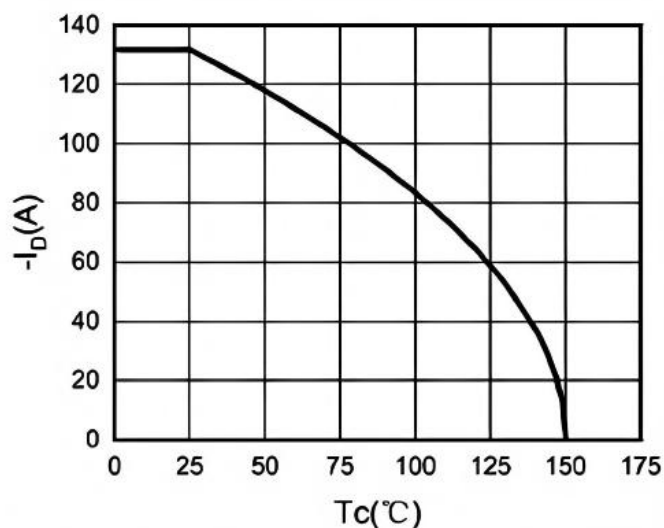
Fig.4 Drain Current
