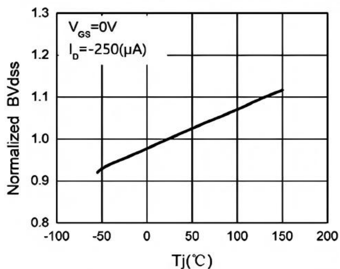
Fig.5 BV DSS vs Junction Temperature
