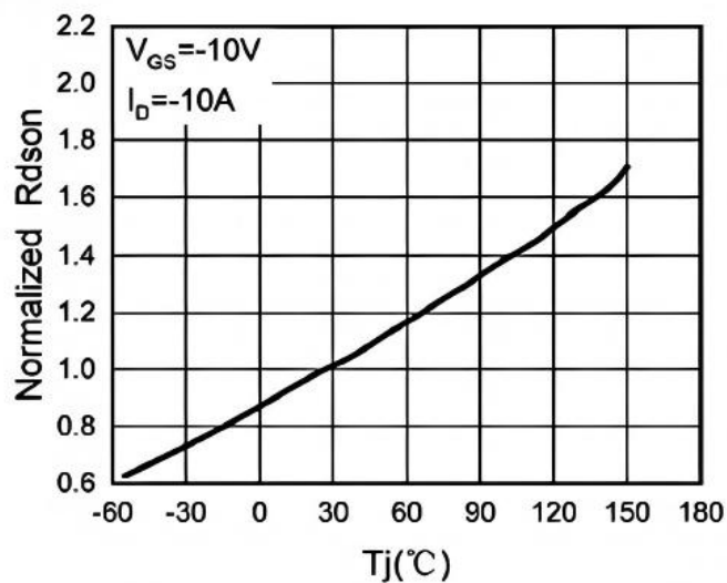
Fig.6 R DS(on) vs Junction
