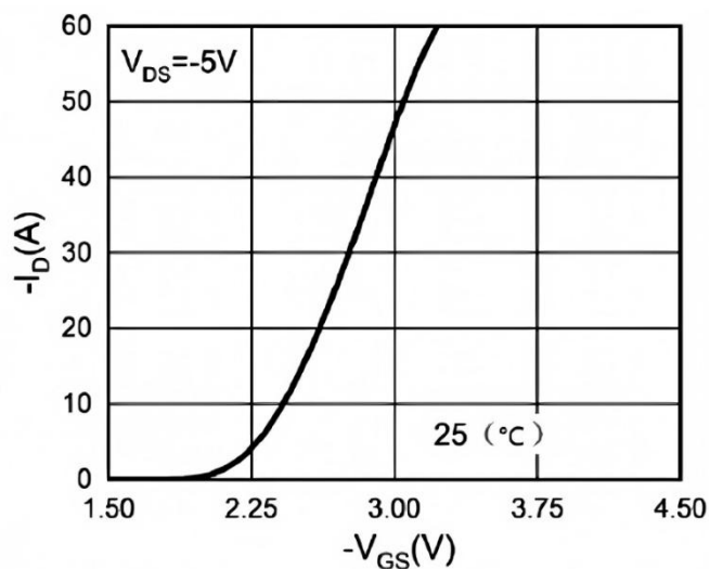
Fig.2 Transfer Characteristics
