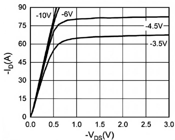
Fig.1 Output Characteristics
